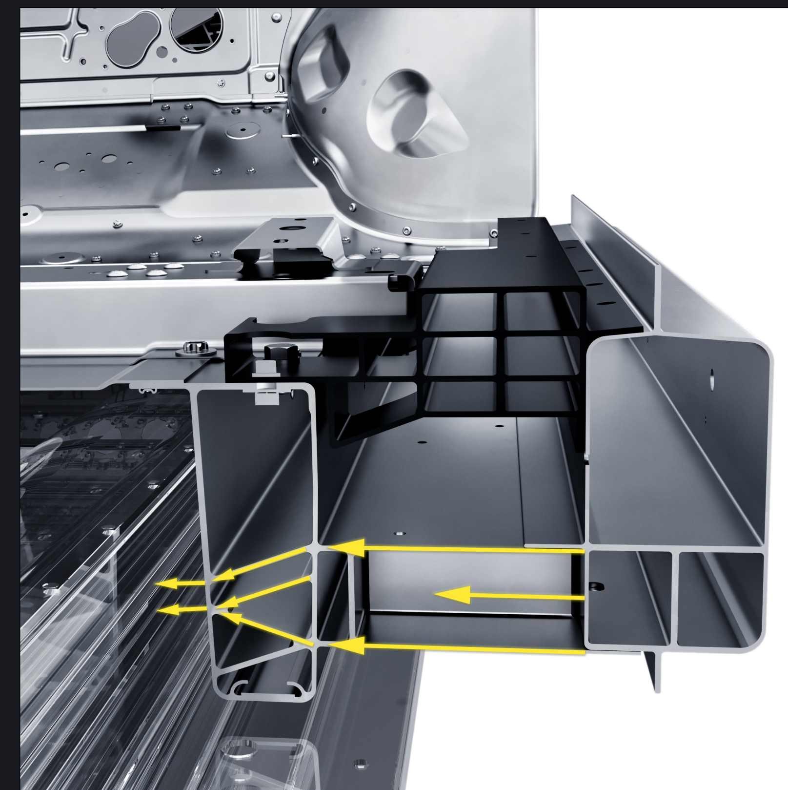
Moat Pack Structure 护城河电池包结构
